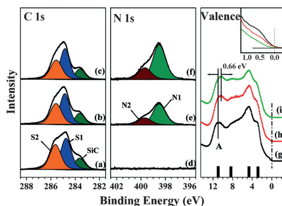
Figure 16. HRPES experiments for graphene functionalization with azidotrimethylsilane: a)–c) C 1s core-level spectra obtained at 320 eV, d)–f) N 1s core-level spectra obtained at 500 eV and g)–i) valence band spectra at 130 eV. Samples: SLG (a,d,g); higher (b,e,h) and lower functionalized EG at 100 °C, (c,f,i). Reprinted from Ref. [66], Copyright 2009 American Chemical Society.
