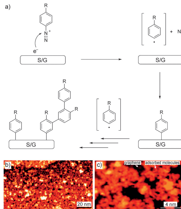
Figure 2. a) Aryl diazonium coupling on S/G. b,c) STM images of SiC/EG-(pNO 2 Ph) at low (b) and high (c) magnification showing the presence of oligomers. Reproduced from Ref. [44], Copyright 2012 American Chemical Society.
