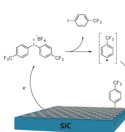
Figure 9. Proposed mechanism for radical functionalization of SiC/EG with trifluoromethylphenyl iodonium based on Ref. [52].
